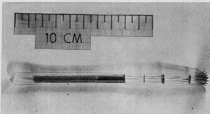
FIG. 1. Resistance thermometer
