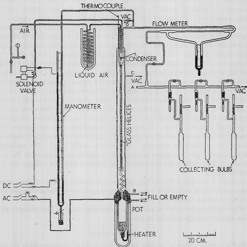
FIG. 6. Low-temperature column
